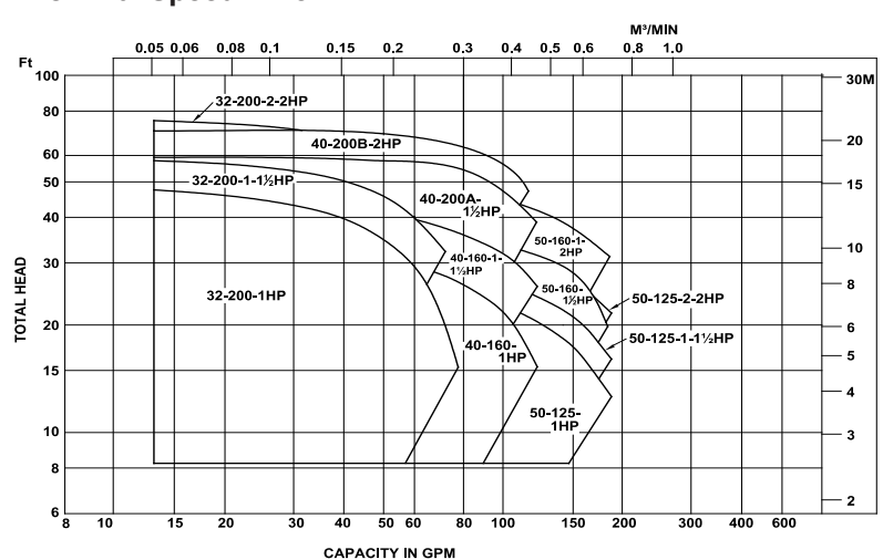
Nominal Speed 1725 RPM
