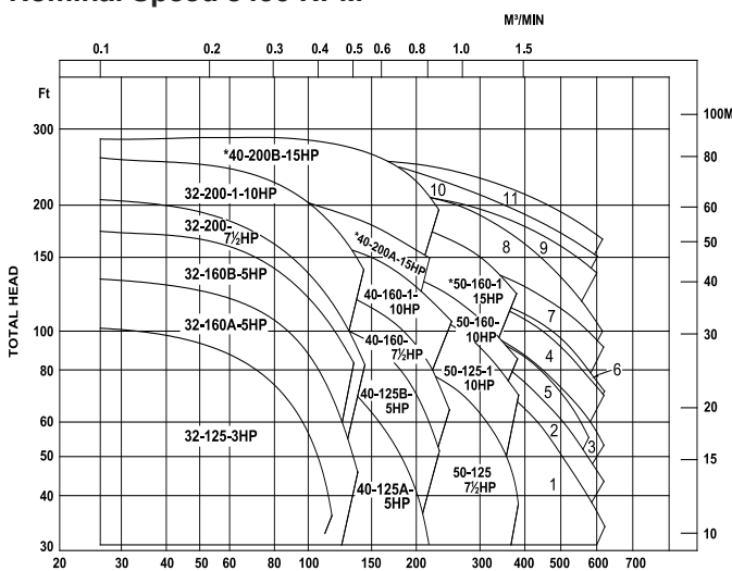
Nominal Speed 3450 RPM
